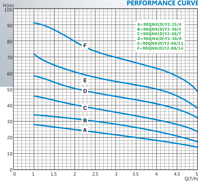
PERFORMANCE CURVE
