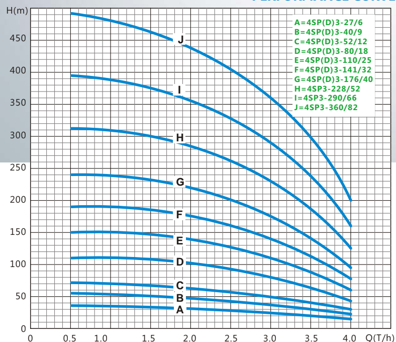
PERFORMANCE CURVE
