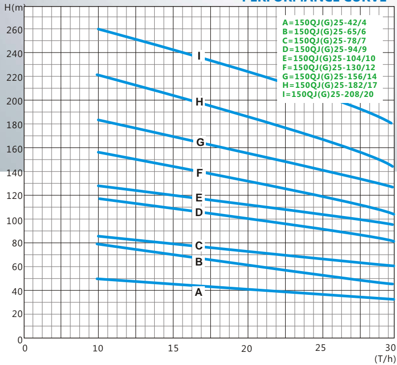
PERFORMANCE CURVE
