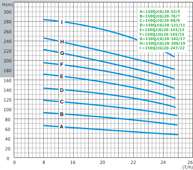
PERFORMANCE CURVE
