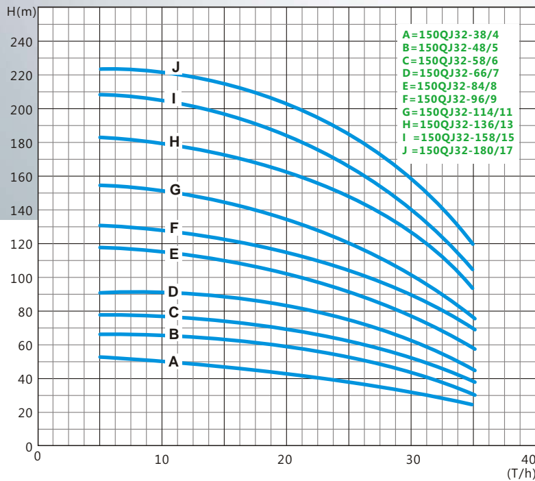
PERFORMANCE CURVE
