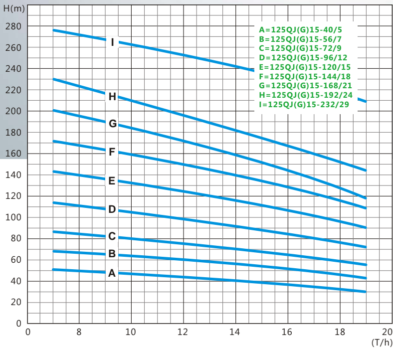
PERFORMANCE CURVE
