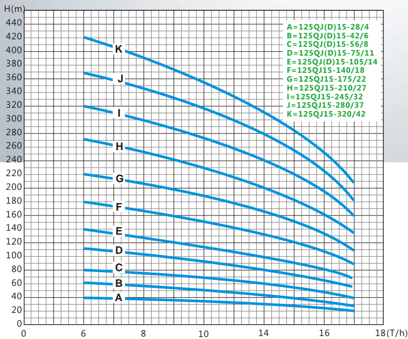
PERFORMANCE CURVE
