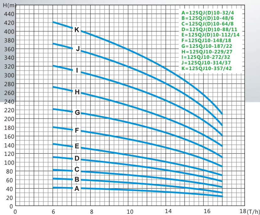
PERFORMANCE CURVE
