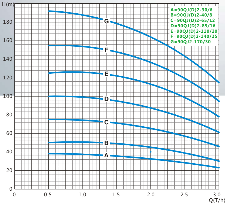
PERFORMANCE CURVE
