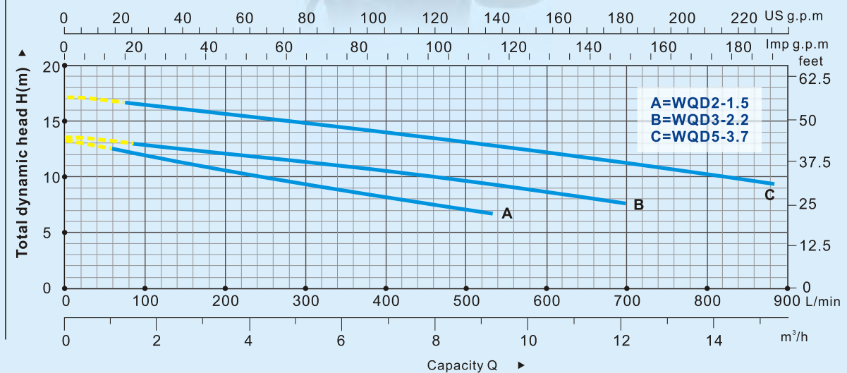
PERFORMANCE CHART AT n=2900 l/min
